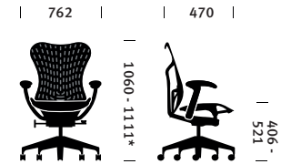
Work Chair with Butterfly Back*
